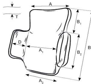
A - Width, A1 - Width, B - Total cushion length, B1 - Headrest length, B2 - Pelottes length, D - Pelottes width, T - Cushion thickness
